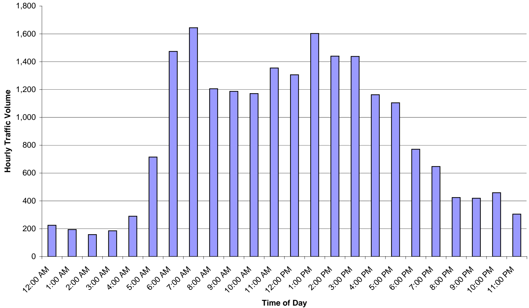
Figure 2.1 24-hour Traffic Volume on Front Street
